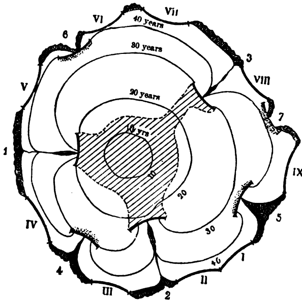
Fig. 383.—Cross-section of a pine first tapped "alive," and then tapped to death.
